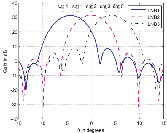
Fig. 2. Antenna patterns of LNBs 1, 2 and 3 fixed on a 35-cm parabolic dish. Satellites depicted in black are desired while the ones in red are interferers.
